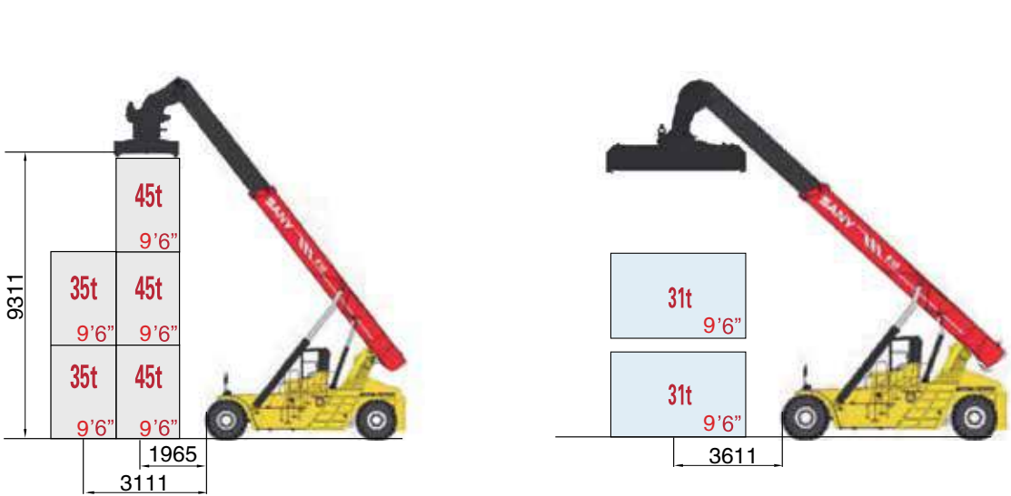
SRSC45T SERIES CONTAINER REACH STACKER
