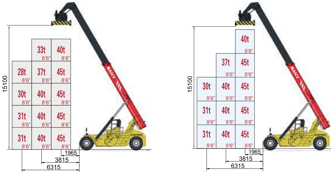
SRSC4540H SERIES HEAVYWEIGHT CONTAINER REACH STACKER
