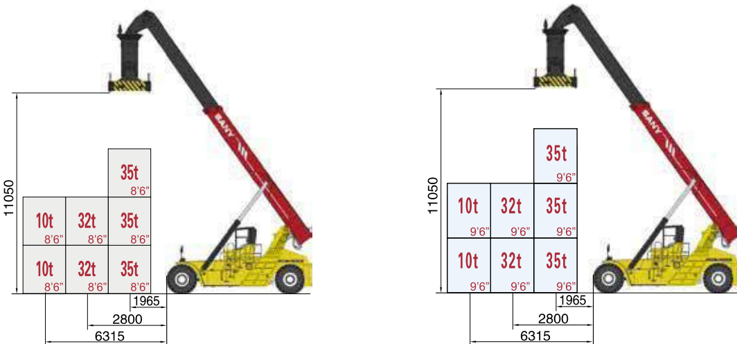
SRSC3532H1-L CONTAINER REACH STACKER NOTE: 2800mm just means that the maximum lifting capacity is 32t at this position, not equal to the distance of the container in the second row.
